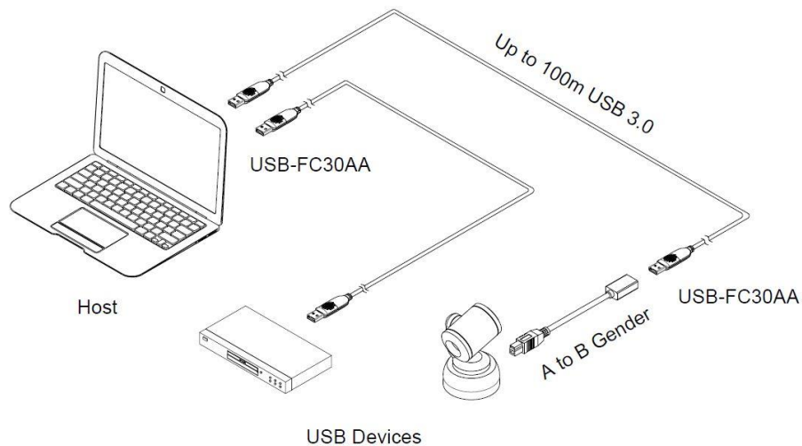
Figure 1 – Overall Connection of USB-FC30AA
